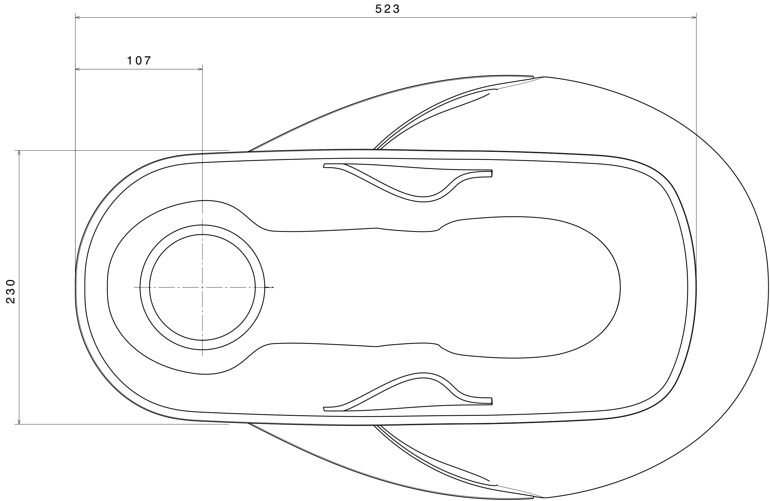
CONCORDE CONCEALED 'S' PAN FOOT PROFILE - 02-09-09 APPROX. DIM'S FOR REFERENCE ONLY
