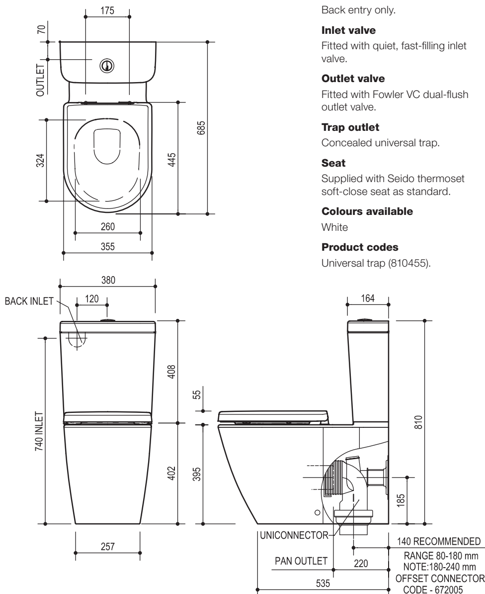
Drawing Scale 1:15
