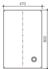
Large Access Panel Single Flush — Bottom Code No.237032
