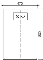
Large Access Panel — Top Code No.237030
